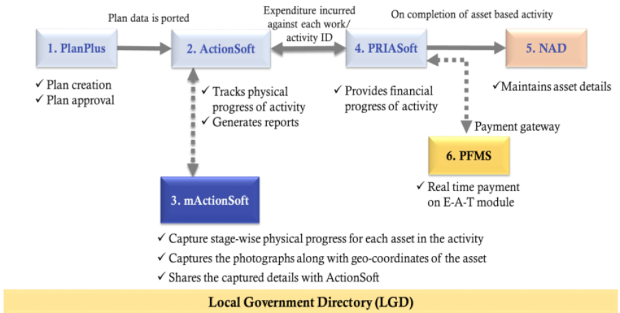
Diagram 5: Architecture of Electronic Fund Management System
